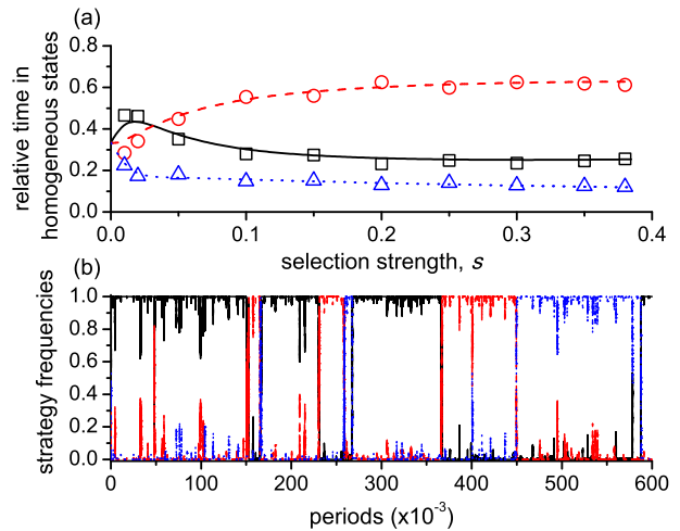
FIG. 6: (Color online.) A population of M = 100 individuals evolving through Moran update. (a) Comparison of the relative times in which the population is in a homogeneous state vs. the selection strength, s , for low mutation rates. Lines represent the analytical estimates obtained in Sec. C 2; symbols represent the results from agent-based simulations. (b) Fractions of each strategy as a function of time as obtained from a realization of an agent-based simulation. Cooperators are represented with a black solid line and squares, defectors with a red dashed line and circles, and jokers with a blue dotted line and triangles. Parameters are n = 5 , r = 3 , d = 0.4 and \mu = 5 \times 10^{-5} . In (b) the selection strength is s = 0.05 .
