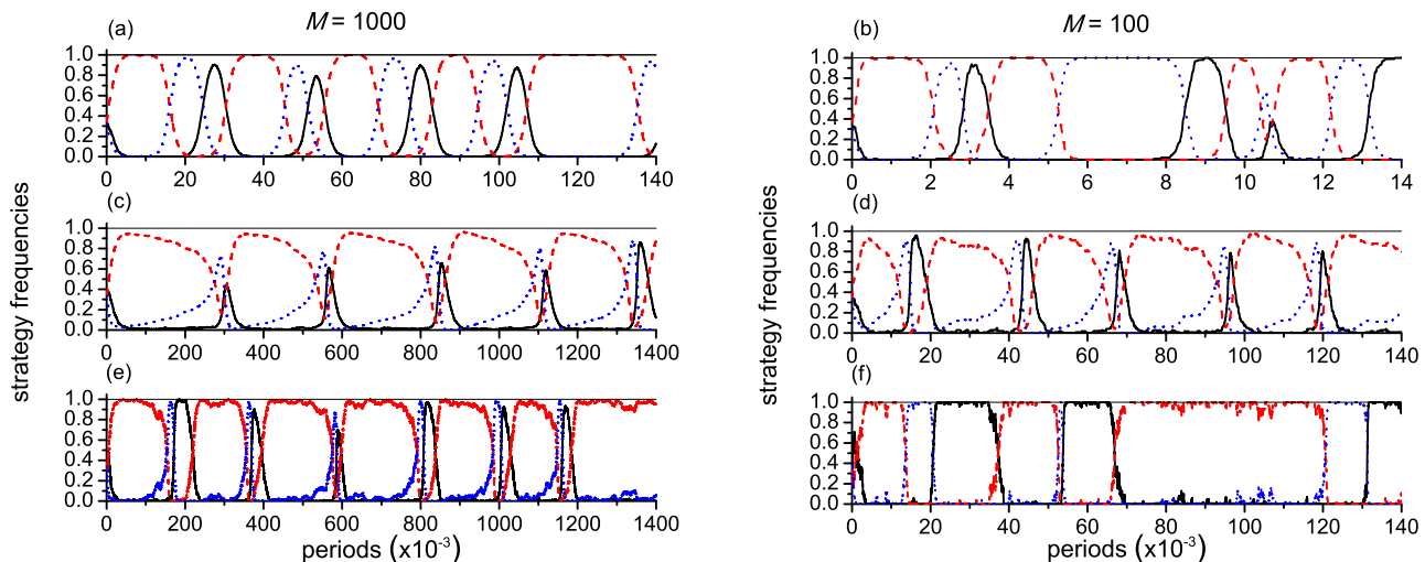
FIG. 2: (Color online.) Time evolution of the frequencies of the three strategies in a population of M = 1000 (left) and M = 100 (right) individuals playing a PG with jokers with different update rules: (a), (b) unconditional imitation, (c), (d) proportional update, and (e), (f) a Moran process. The presence of jokers induces a cyclic behavior irrespective of the update rule and the population size, as long as the mutation rate \mu > 0 . Black solid lines: cooperators, red dashed lines: defectors, and blue dotted lines: jokers. One period corresponds to one updating event according to the evolutionary rule used. Parameters n = 5, r = 3, d = 0.4, \mu = 0.001 ; in (a)-(d) s = 1 , in (e),(f) s = 0.38 .
