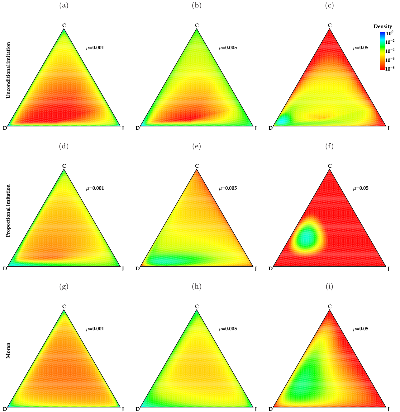
FIG. 7: Density plots for the probability of finding the system in each population state as obtained by solving numerically Eq. (8). First row corresponds to unconditional imitation, second row to proportional imitation, third row to a Moran process. In each case mutations increase left to right. In all three cases low mutation rates ( \mu ) yield high probabilities near the boundaries of the simplexes, specially near the corners, corresponding to cyclic transitions between homogeneous states. Increasing \mu increases the probability to find the system near homogeneous defective populations. For high \mu an attractive point appears close to the D corner which goes away from it upon increasing \mu . Parameters are n = 5, r = 3, d = 0.4 ; the selection strength is s = 1 in the first and second rows, s = 0.38 in the third. Mutation rates have been chosen as in Fig. 1 and appear near each simplex. Densities are plotted using a logarithmic scale.
