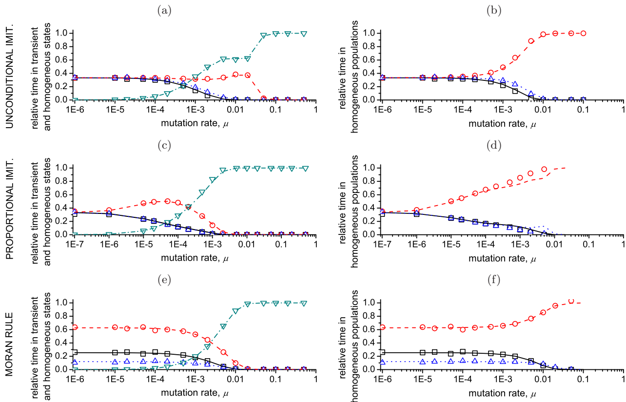
FIG. 3: (Color online.) Relative times spent in homogeneous as well as in transient states in a population of M = 100 individuals. For practical purposes, a state is considered homogeneous if more than 95% of individuals belong to the same strategy. Symbols are the result of agent-based simulations; lines are obtained from the solution of Eqs. (17)–(18). Results for cooperators are represented with (black) squares and solid lines, those for defectors with (red) circles and dashed lines, and those for jokers with (blue) triangles and dotted lines. Panels (a), (c) and (e) also show (with inverted triangles and dashed-dotted lines) the fraction of time spent in transient states. Panels (b), (d) and (f) show the fractions of the time spent in each of the three homogeneous states relative to the total time spent in homogeneous states. Panels (a) and (b) correspond to unconditional imitation, panels (c) and (d) to proportional update, and panels (e) and (f) to a Moran rule. We can see that high mutation rates promote defection over the other two strategies. Parameters used are n = 5 , r = 3 , d = 0.4 ; selection strength is s = 1 in (a)–(d) and s = 0.38 in (e) and (f).
