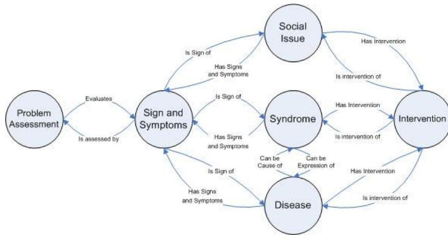
Fig. 1. Case Profile Ontology: main classes and properties.
