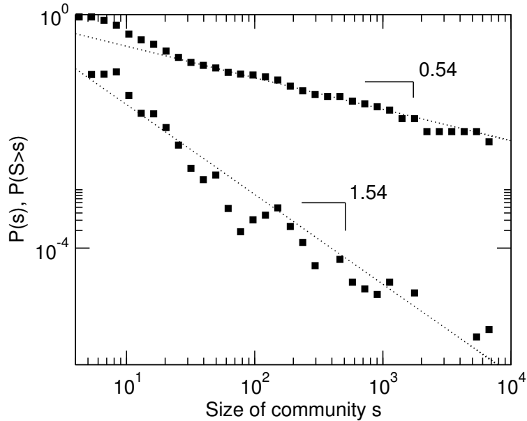
FIG. 3: The size distribution of community sizes in the ArXiv collaboration network. The cumulative distribution follows a power law over several decades with exponent -0.5 . The non-cumulative distribution, although noisier seems to follow a power law with exponent with around -1.5 as expected.
