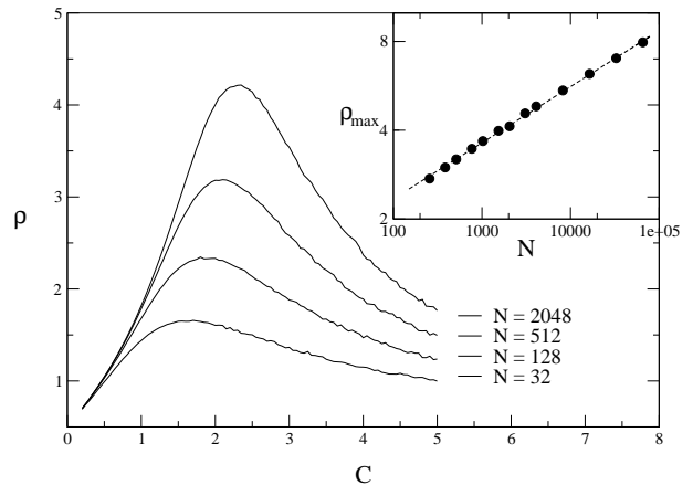
FIG. 4. \rho as a function of C for several system sizes. At the extremes C \rightarrow 0 and C \rightarrow \infty , the value of \rho goes to \langle \Delta_i \rangle = \lambda = 1/2 . There is a peak, \rho_{max} , that diverges in thermodynamic limit N \rightarrow \infty . In the inset we plot \rho_{max} against system size N . Dashed line shows the fit \rho_{max} \sim N^{0.20(1)} .
