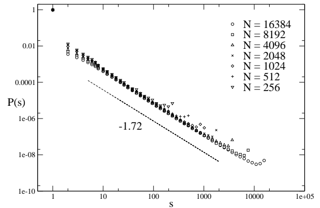
FIG. 2. Plot of the probability density of having a technological avalanche of size s for C = 3 in log-log scale. We find that P(s) \sim s^{-\tau} with \tau = 1.72 . The peaks at the end of each curve are due to finite size effects. Numerical simulations have been averaged over 10^8 avalanches
