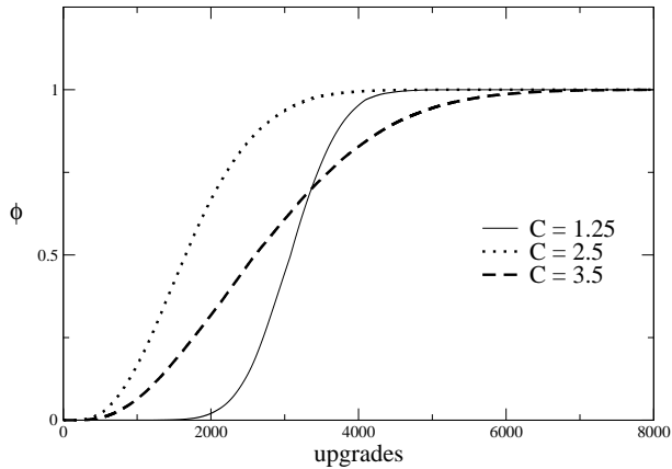
FIG. 3. Evolution of the fraction of agents with a > a_{th} = 3 for N = 1024 and several values of C as the number of upgrades increases. Numerical simulations have been averaged over 1000 initial configurations. In this example the curve for C = 2.5 is always above the others.
