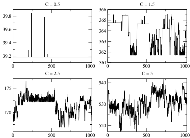
FIG. 1. Technological profiles ( N = 1024 ) for several values of C in the stationary state. For C = 0.5 the profile is almost flat (synchronized state) with everybody sharing the same technology. As we increase C the profile gets noisier and plateaus (agents that, at some point have shared the same technology) become less common. For C = 5 the technological profile is very random.
