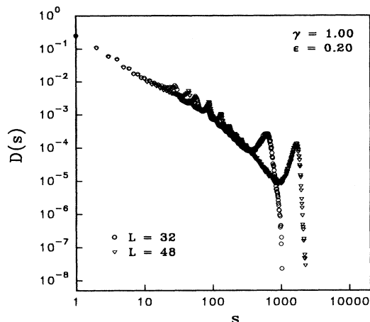
FIG. 2. Distribution of avalanche sizes in region B.
