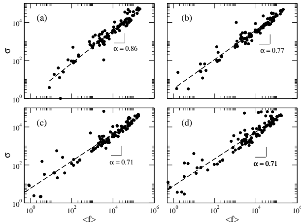
FIG. 4: Scaling relations between \sigma and \langle f \rangle for the 112 Abilene backbone router Interfaces. Analysis performed during (a) two days, (b) one week, (c) one month and (d) two months, finishing all them in November 15th of 2005. The time window length P is fixed to 5 minutes.
