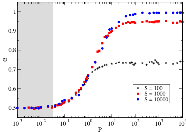
FIG. 1: (Color online) Value of the exponent \alpha versus the time window length P in which averages are performed, for a fixed \lambda_*^{ef} = 1/3 and different values of the persistence of packets in the network S . The shadowed area highlights the region of P in which the exponent \alpha = 1/2 always appears. The simulation is performed in a scale-free network with exponent for the degree distribution \gamma = 3 of 1000 nodes [20]. We have observed the same results for larger SF networks at a subset of values of P , however the computational cost for the whole set of P values used in the plot becomes prohibitive.
