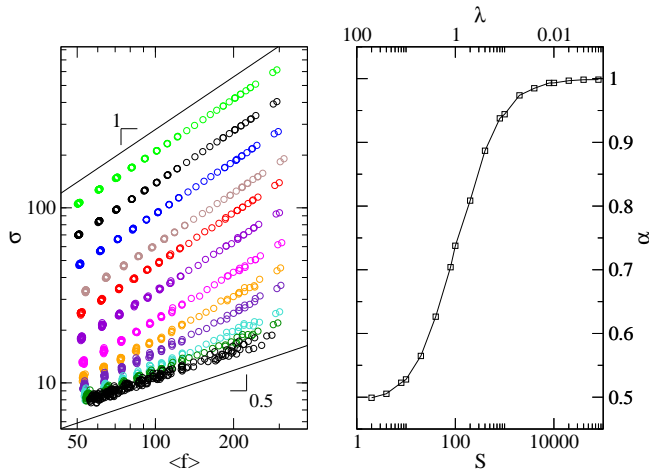
FIG. 2: (Color online) Left: Plot \sigma versus \langle f \rangle for different realization of \lambda and S maintaining its product constant. The simulation is performed in a scale-free network with exponent for the degree distribution \gamma = 3 of 1000 nodes [20]. We fixed \mathcal{T} = \lambda S = 100 . Right: Plot of the \alpha exponent for \lambda S = 100 . Other values of \lambda S have produced equivalent results, shifted to a different region of \langle f \rangle .
