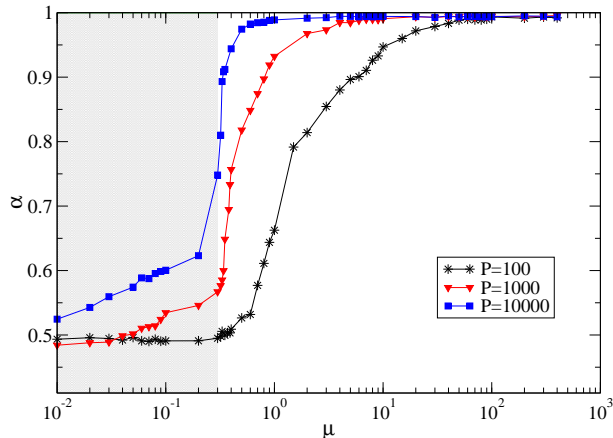
FIG. 3: (Color online) Scaling exponent \alpha as a function of the time service \mu , for three different time window lengths, and for \lambda_*^{ef} = 1/3 . Shaded area highlights the region where congestion starts at nodes with \lambda_*^{ef} = 1/3 .
